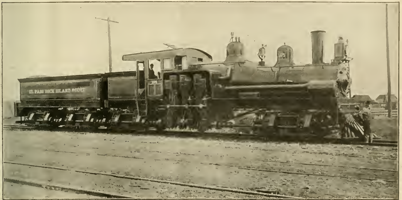
LIMA SHAY LOCOMOTIVE.
